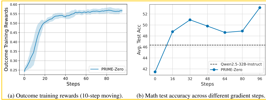
Figure 13: “Zero” RL from Qwen2.5-32B-Base. RL from a 32B base model shows more promising gain, surpassing the instruct version within 16 steps.
