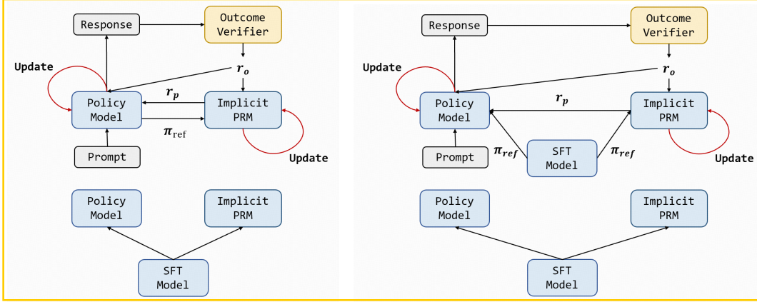
(a) Policy ref: We use the policy logprob as \pi_{ref} for PRM. (b) SFT ref: We retain the initial policy to provide \pi_{ref} for PRM and KL.
