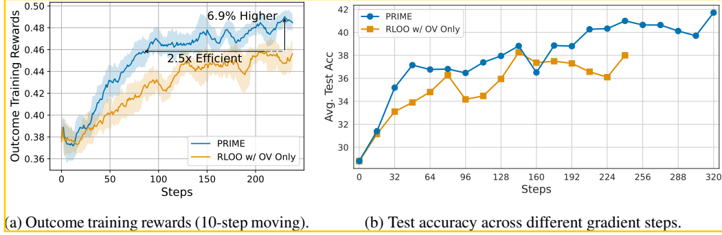
Figure 4: The effect of dense reward. We compare PRIME and RLOO with outcome verifier (OV). Dense rewards in PRIME lead to 2.5x sample efficiency and 6.9% performance improvement. PRIME also substantially outperforms RLOO on downstream tasks.
